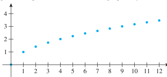
Graph of g where g(n) = n^{1/2} for each nonnegative integer n
