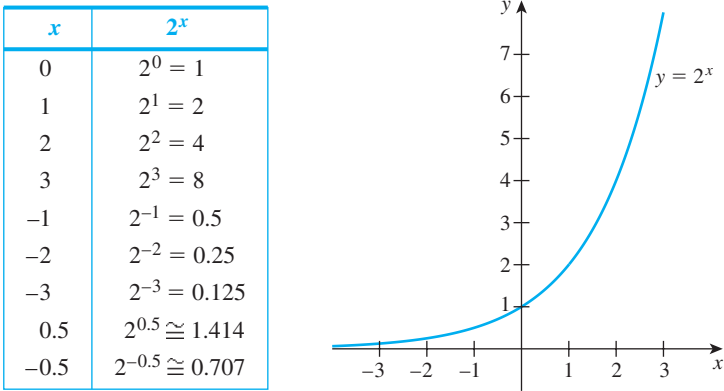
FIGURE 11.4.1 The Exponential Function with Base 2
