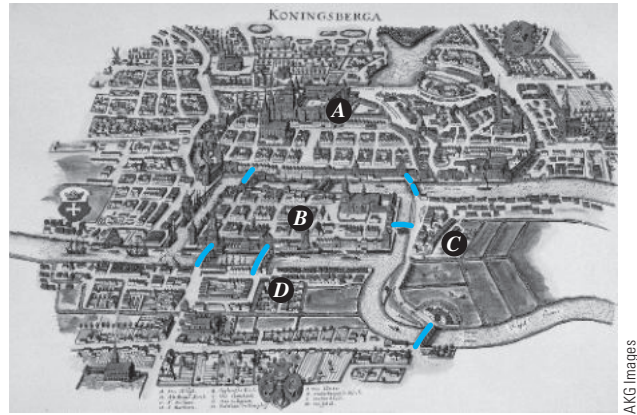
FIGURE 10.1.1 The Seven Bridges of Königsberg
