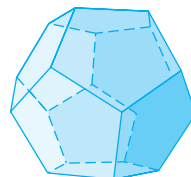
FIGURE 10.1.7 Dodecahedron
