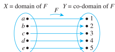
FIGURE 7.2.5 An Arrow Diagram for a One-to-One Correspondence
