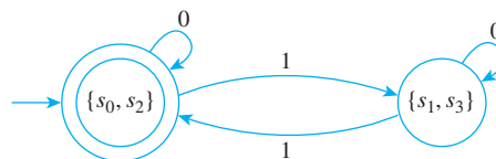
FIGURE 12.3.2 Transition Diagram for \bar{A}
