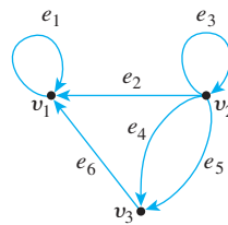
Directed Graph G (a)
