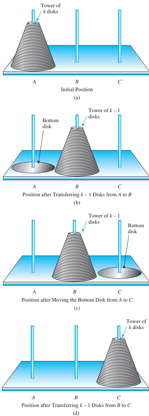
FIGURE 5.6.2 Moves for the Tower of Hanoi
